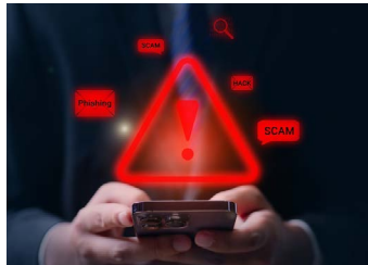
Phishing attacks
